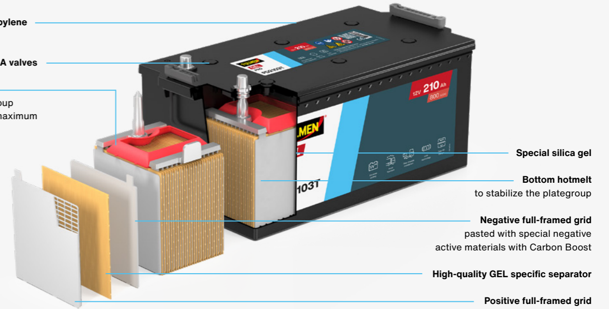
Image shows the FD2103T type
