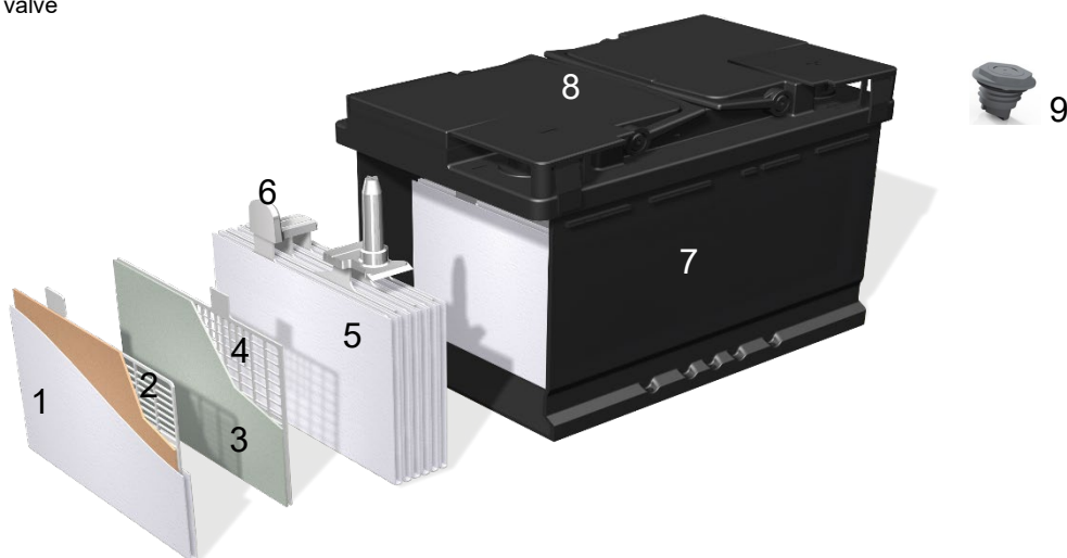
Figure 1 - Conceptual design of a prismatic VRLA-AGM lead acid battery
